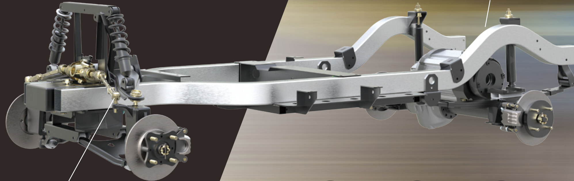
DOUBLE WISHBONE INDEPENDENT SUSPENSION
